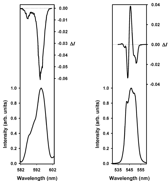
Figure 4. Circularly polarized luminescence (upper curves) and total luminescence (lower curves) spectra of the ^5\text{D}_0 \rightarrow ^7\text{F}_1 transition of [\text{Eu}(\text{H1})(\text{H}_2\text{O})] (left) and ^5\text{D}_4 \rightarrow ^7\text{F}_5 transition of [\text{Tb}(\text{H2})] (right) in saturated aqueous solutions at pH 7.4 (0.1 M Tris buffer) and 295 K, upon excitation at 360 and 350 nm, respectively.
