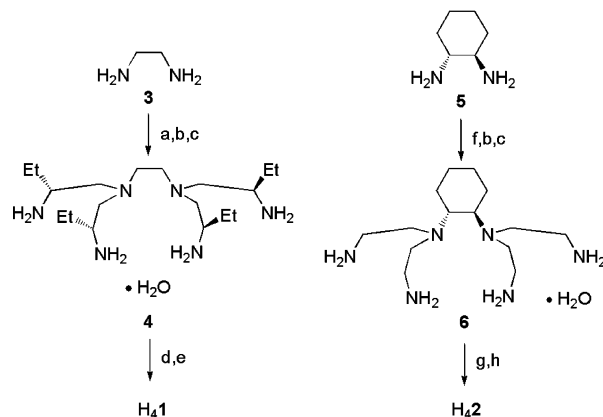
Figure 1. Enantiopure, octadentate ligands.
